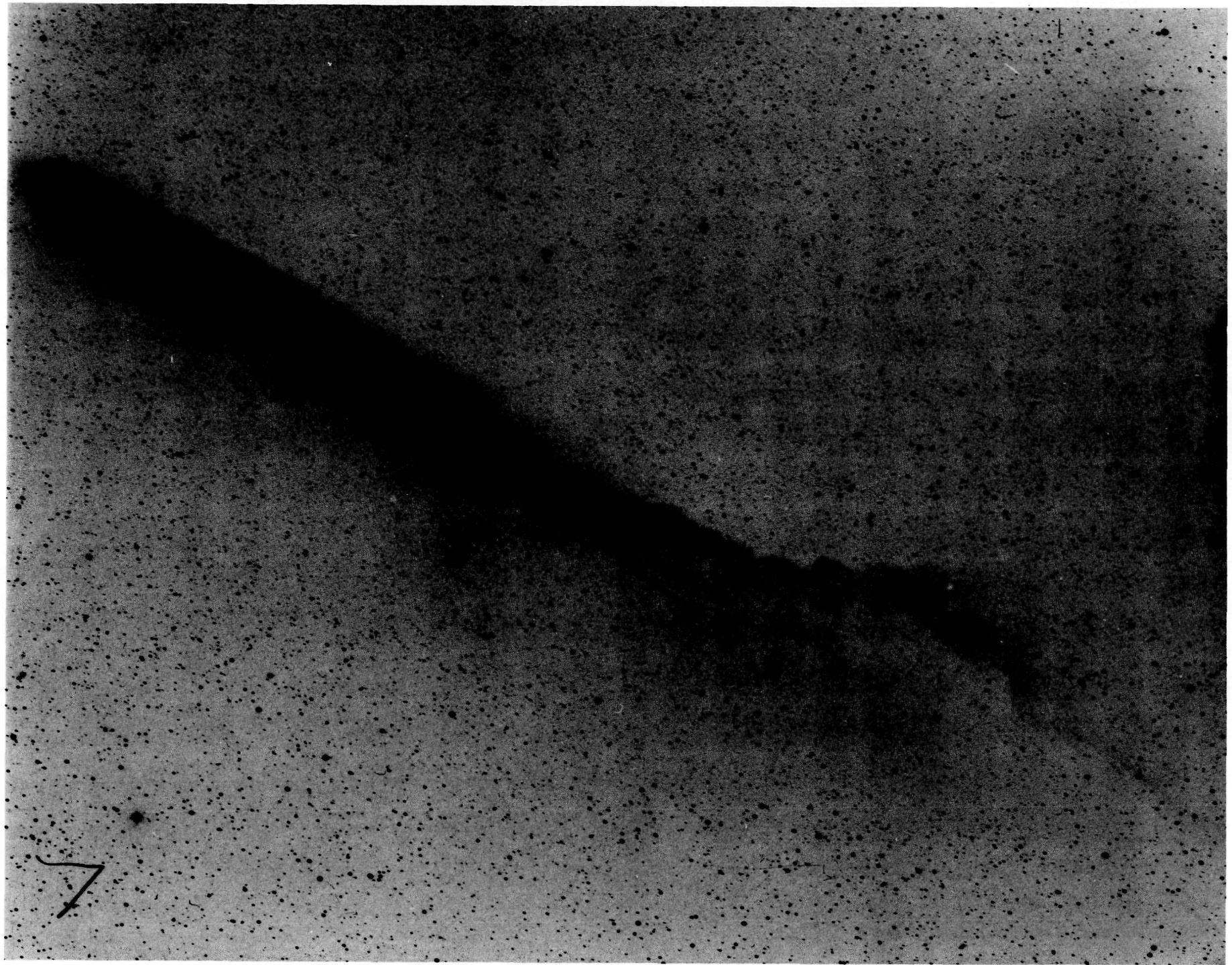
Figure 5. JOCR photograph of comet Kohoutek on January 20, 1974.
